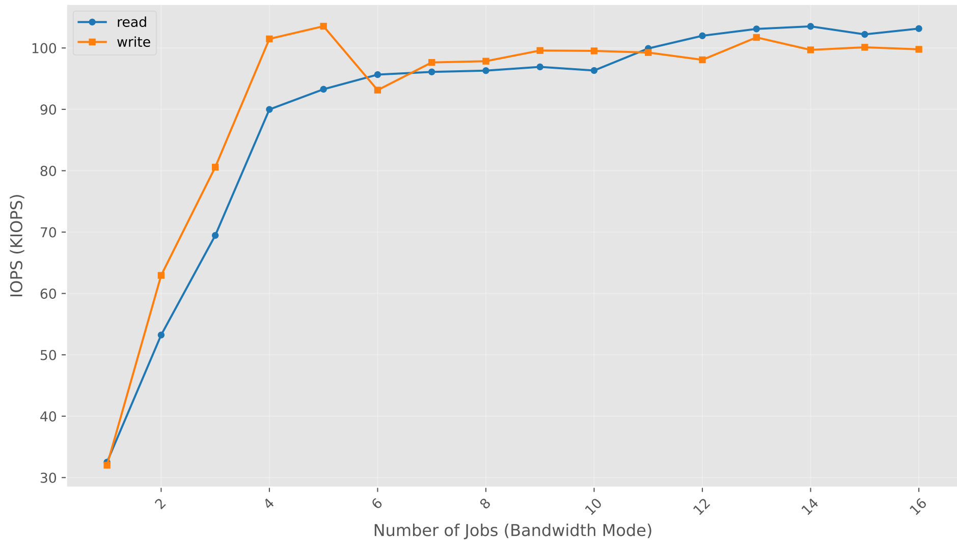
IOPS vs Number of Jobs (Bandwidth Mode)
